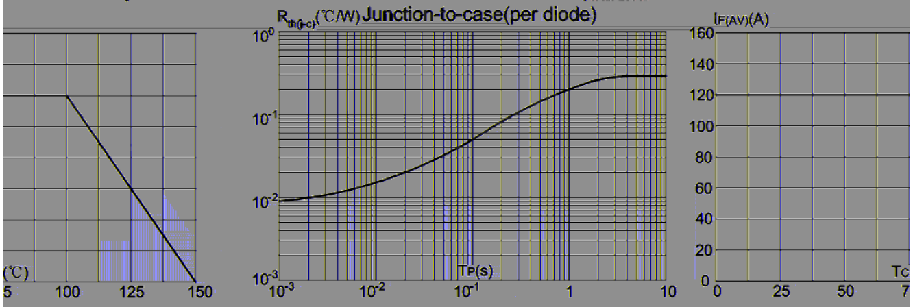
FIG 4: Maximum transient thermal impedance
