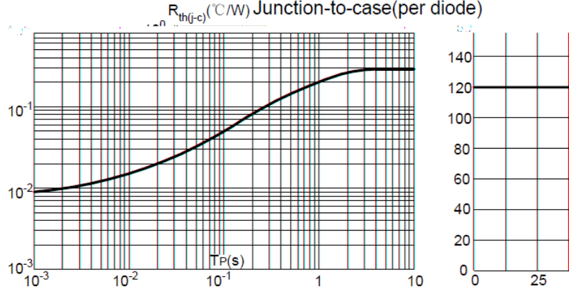
FIG.4: Maximum transient thermal impedance
