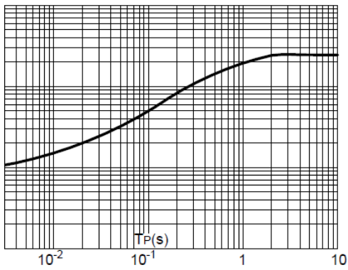
Maximum transient thermal impedance C/W) Junction-to-case(per diode)
