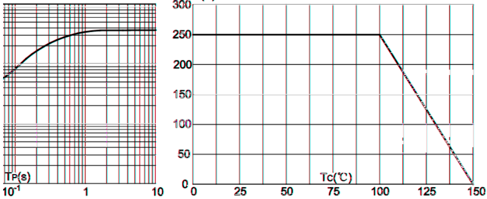
FIG 3: Forward current vs. case temperature
