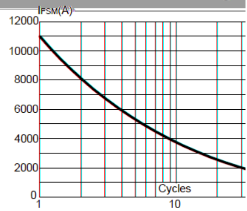
FIG.2: Peak on-state surge current
