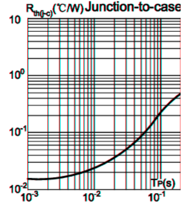
FIG.4: Maximum transient thermal impedance
