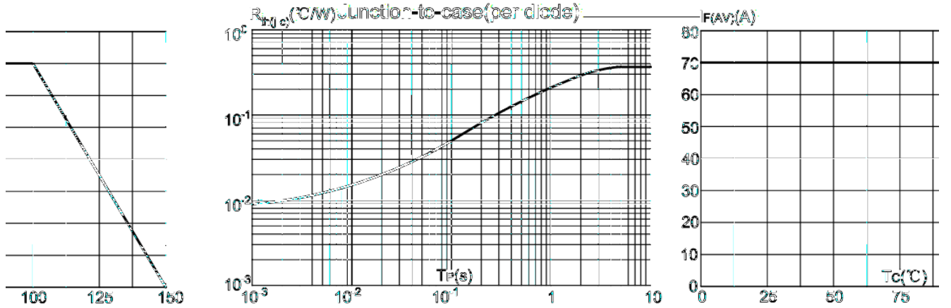
FIG.3: Thermal resistance (per diode)
