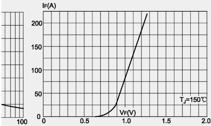
FIG.1: Forward characteristic (acrossed)
