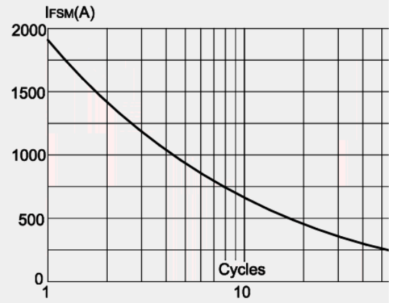
FIG.2: Pulse reverse current vs. pulse width
